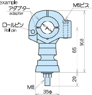
Mounting example
