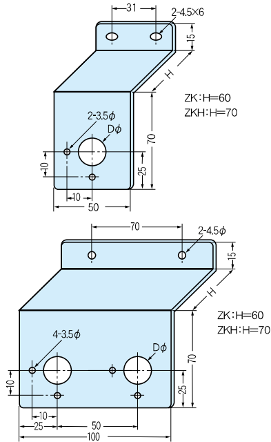
Mounting example
