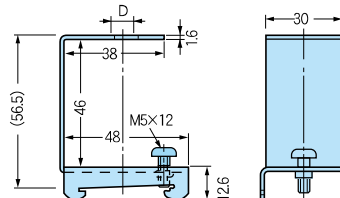
DIN rail mounted toggle switch stand
