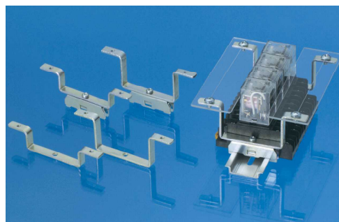
Mounting example
